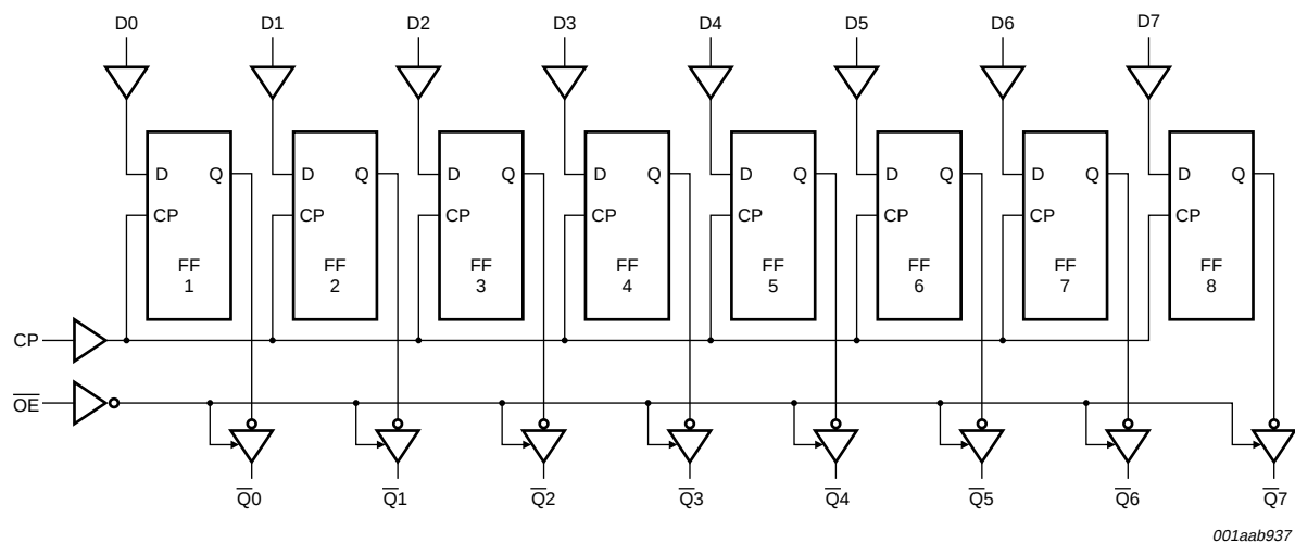
Fig 4. Logic diagram
